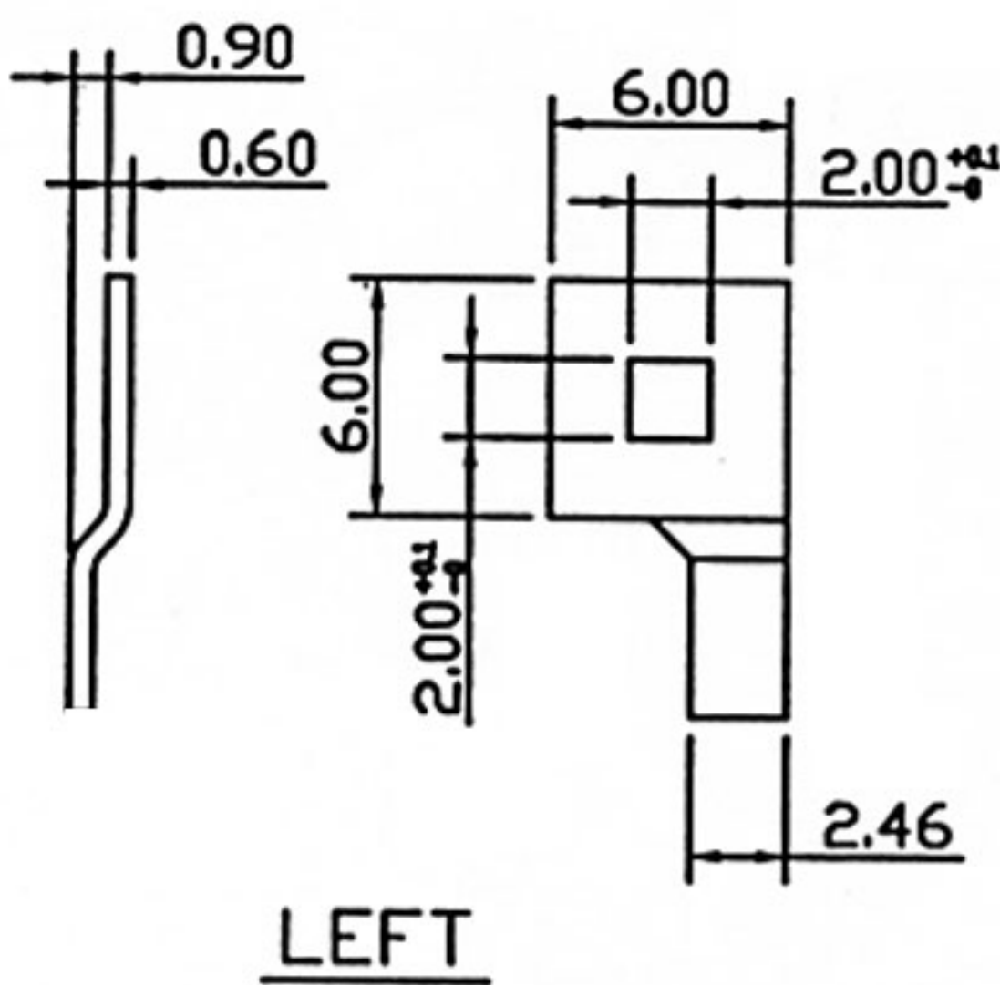
DETAIL "A" 2:1
