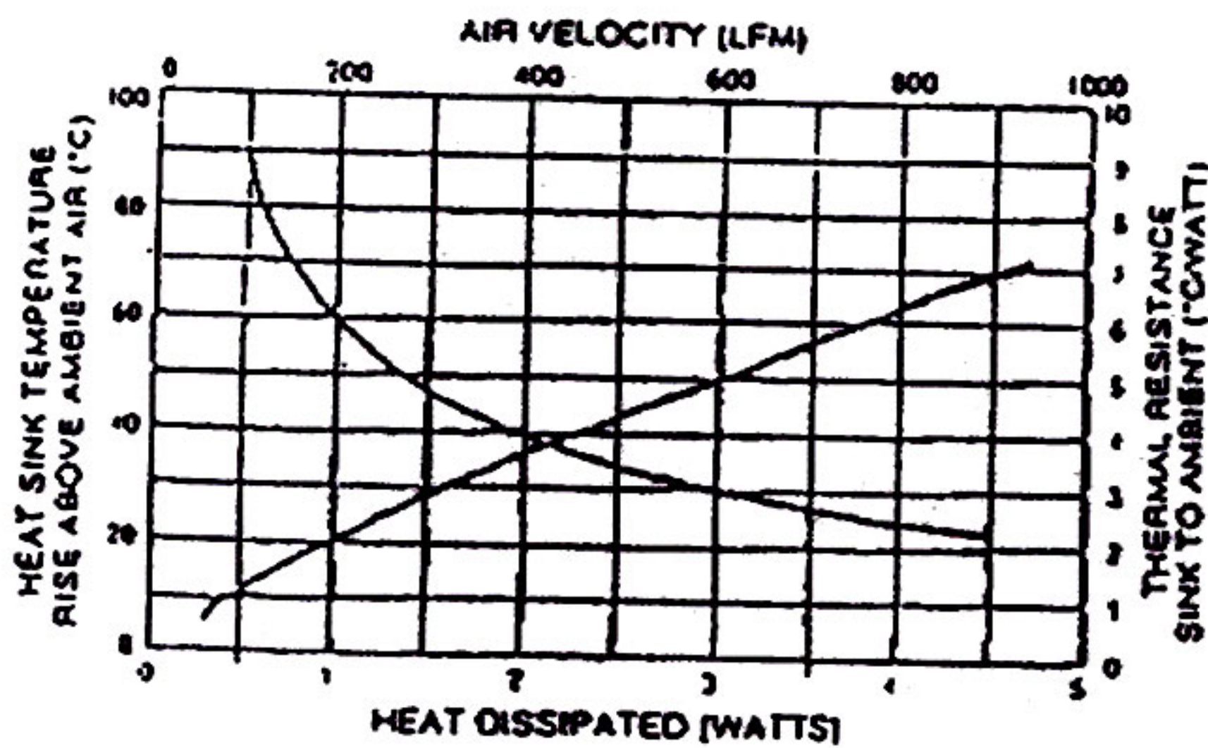
NATURAL AND FORCED CONVECTION CHARACTERISTICS
